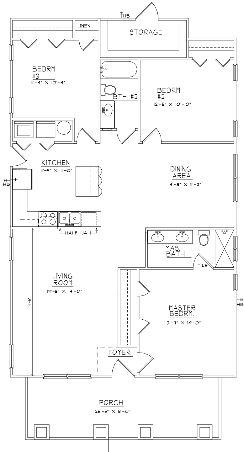
FLOOR PLAN
