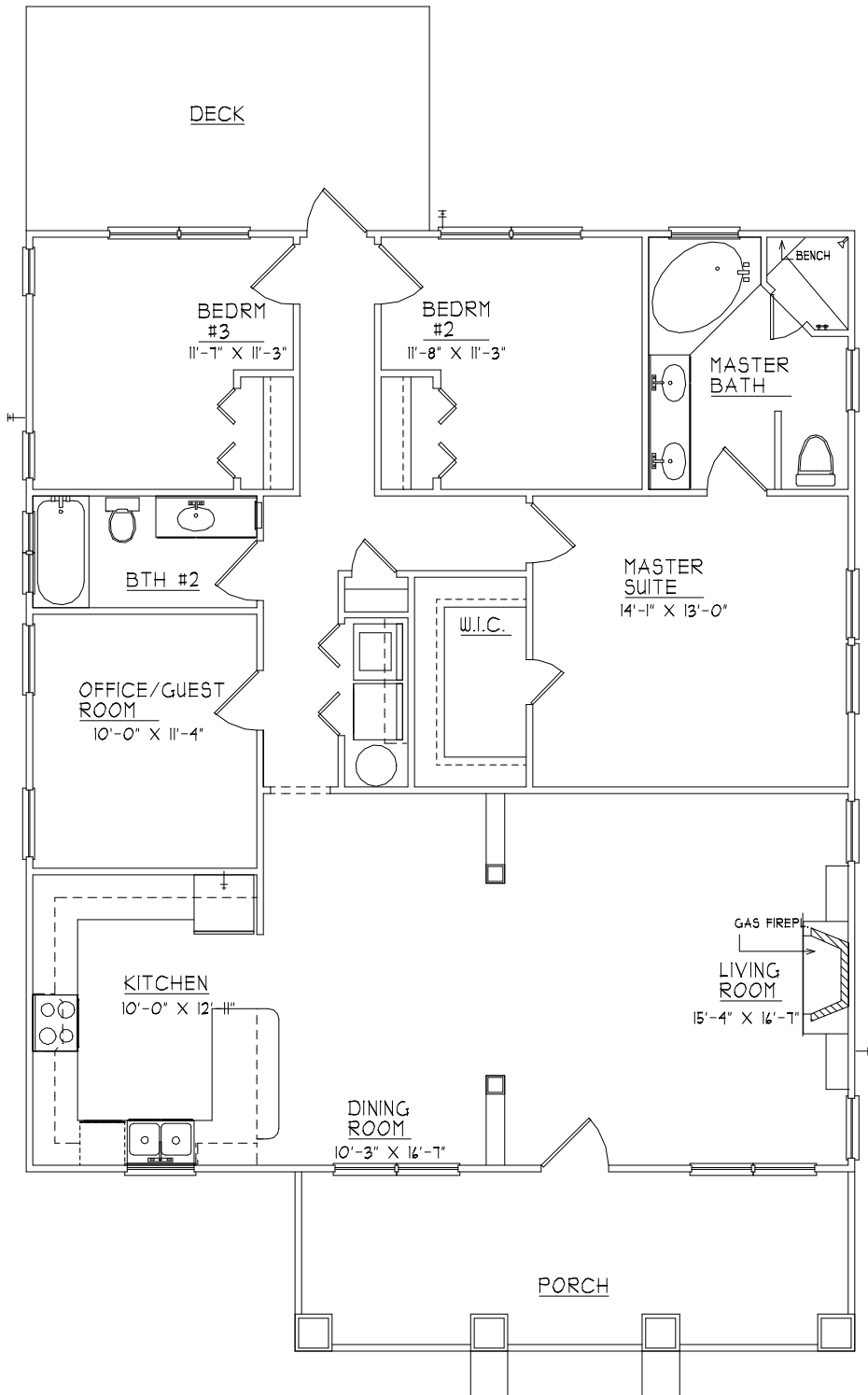
FLOOR PLAN
