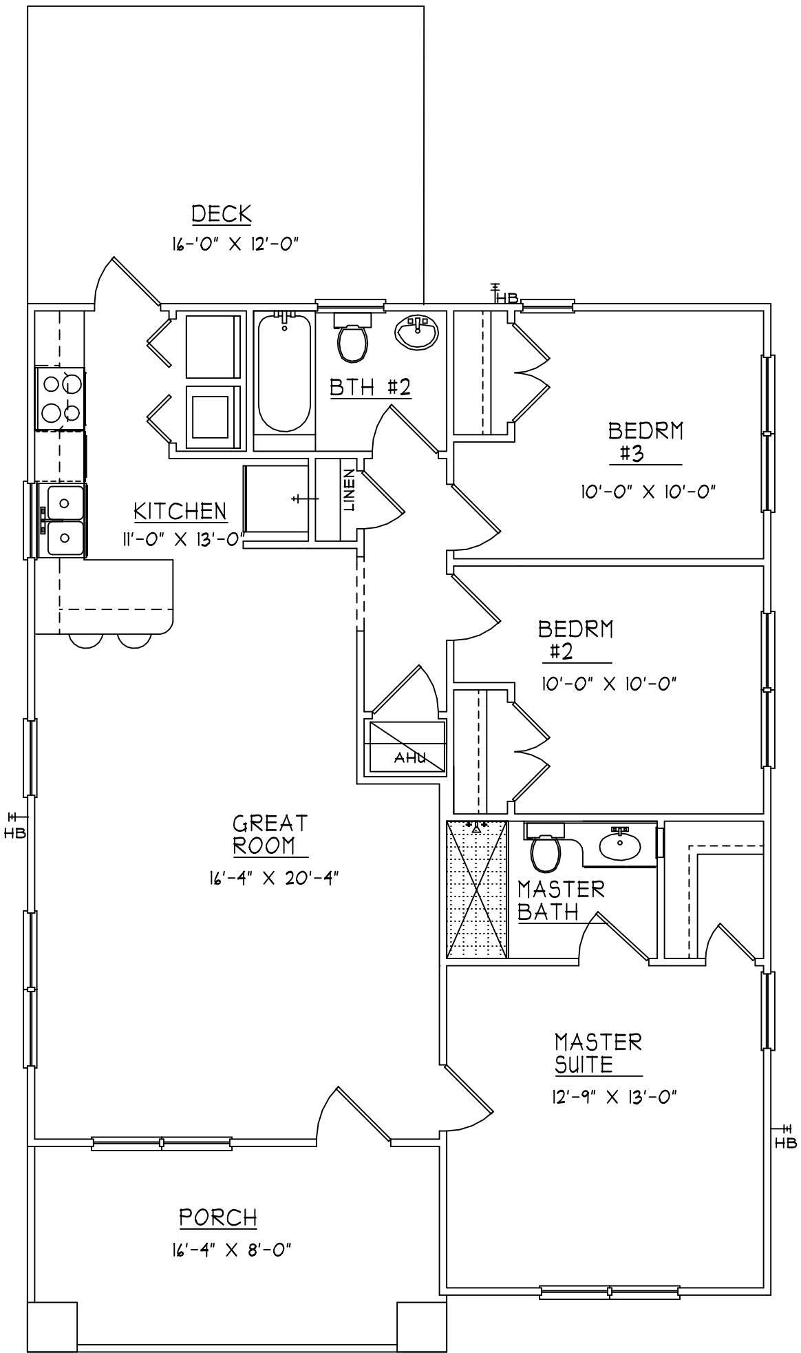
FLOOR PLAN 1084 SQ. FT.
