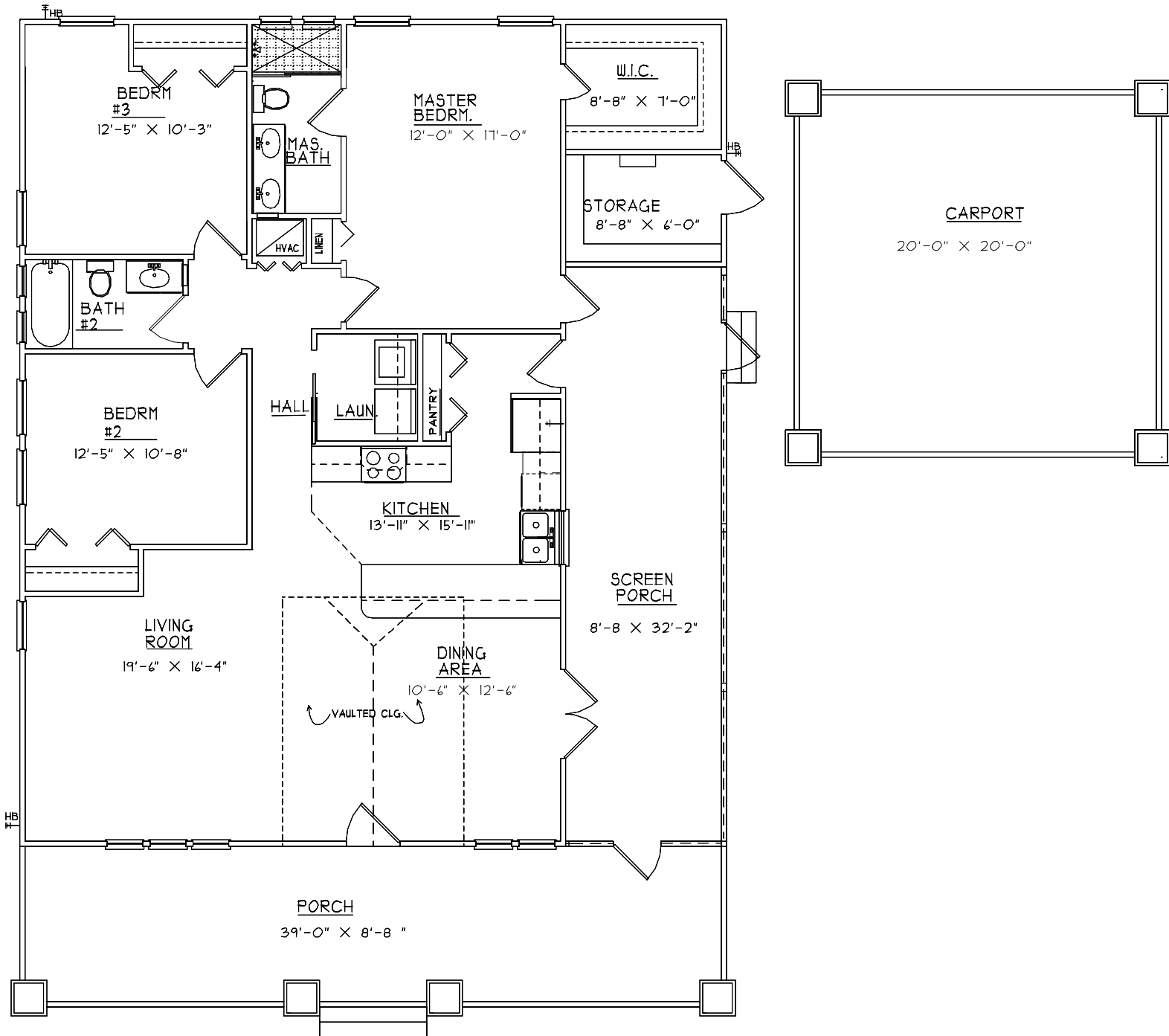
FLOOR PLAN
