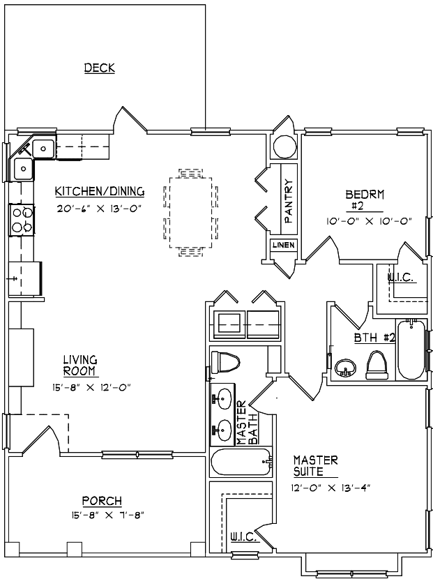
ALT. FLOOR PLAN
