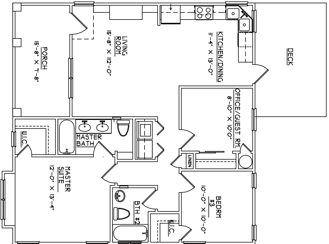
FLOOR PLAN 1040 SQ.FT.
