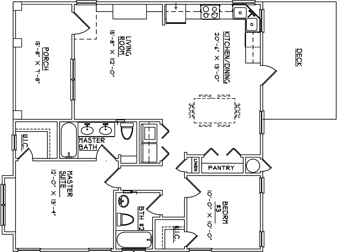
ALT. FLOOR PLAN 1040 SQ. FT.
