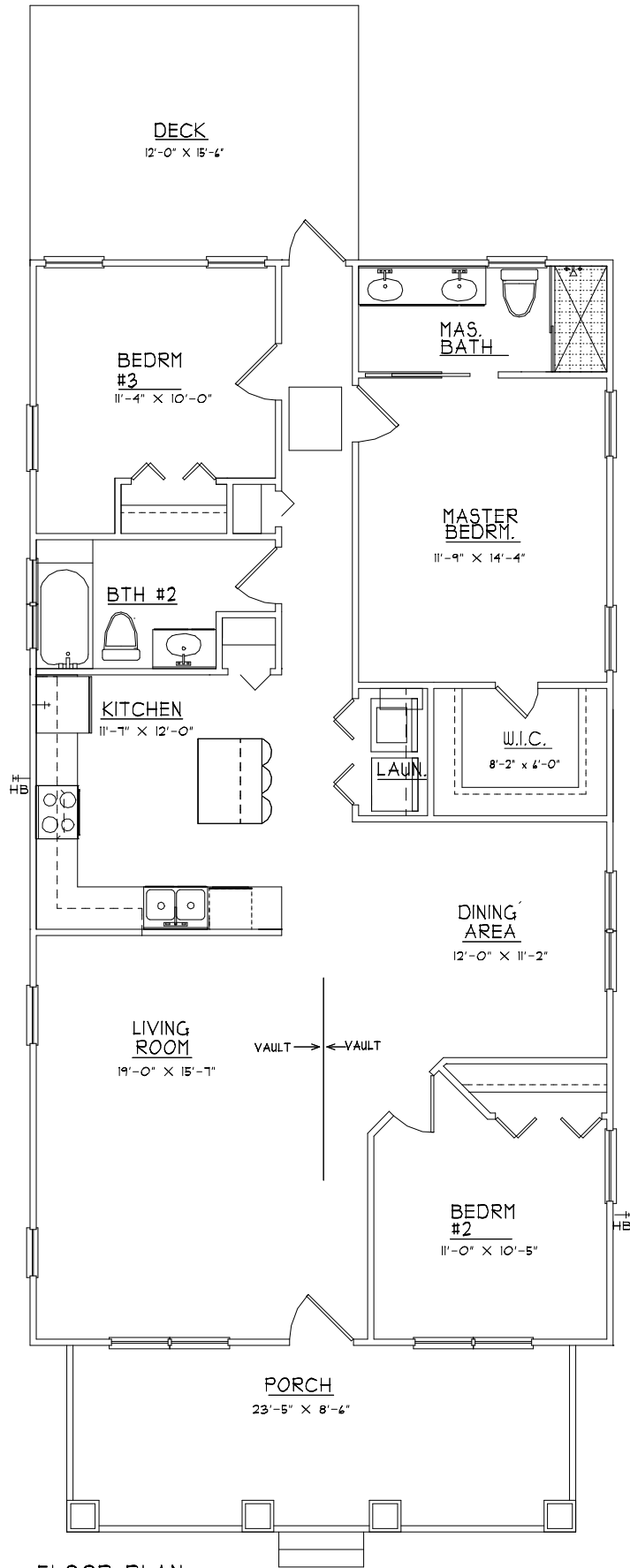
FLOOR PLAN
