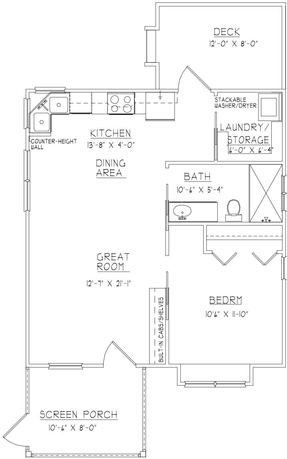
FLOOR PLAN
