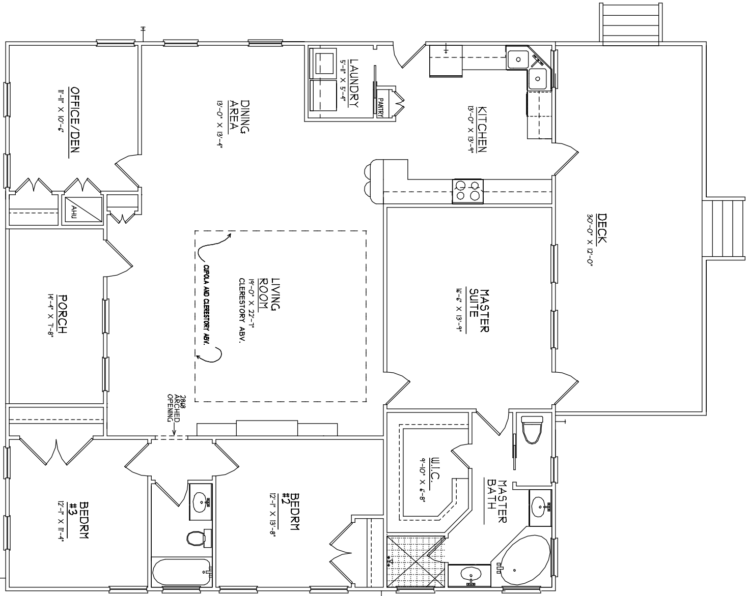
FLOOR PLAN
