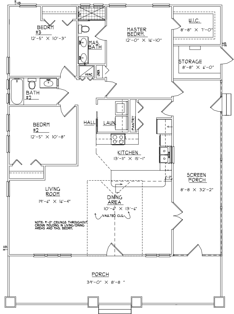
ALTERNATE FLOOR PLAN W/ DETACHED CARPORT TO RIGHT OF HOUSE
