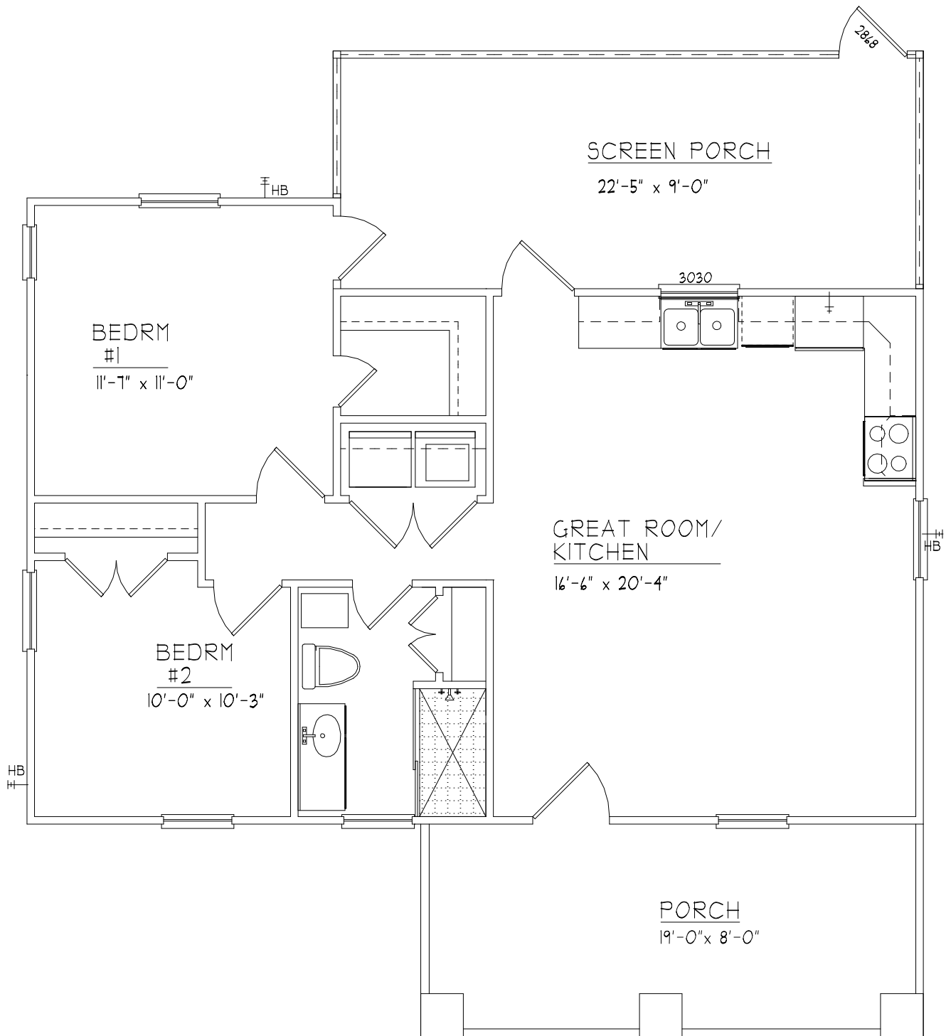
FLOOR PLAN 715 SQ. FT.
