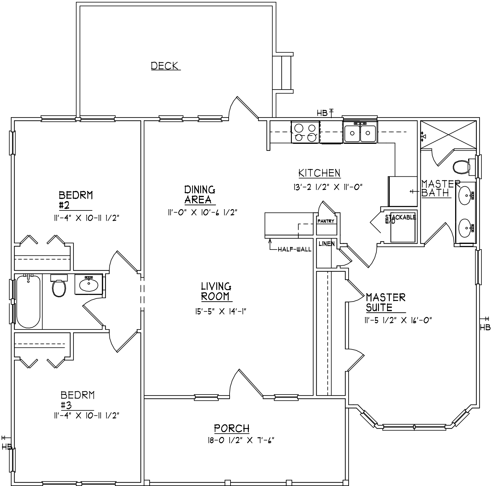
FLOOR PLAN 1201 SQ. FT.
