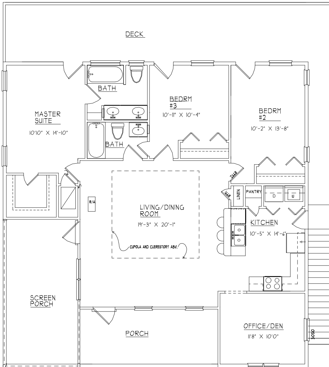
FLOOR PLAN
