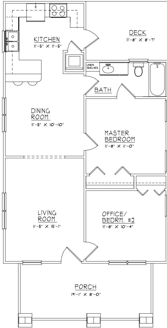
FLOOR PLAN
