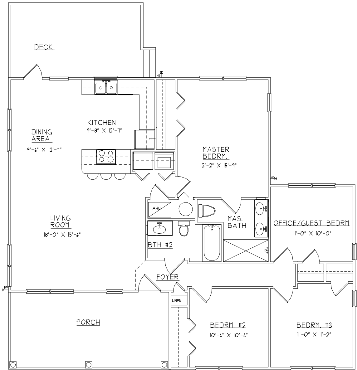
FLOOR PLAN
