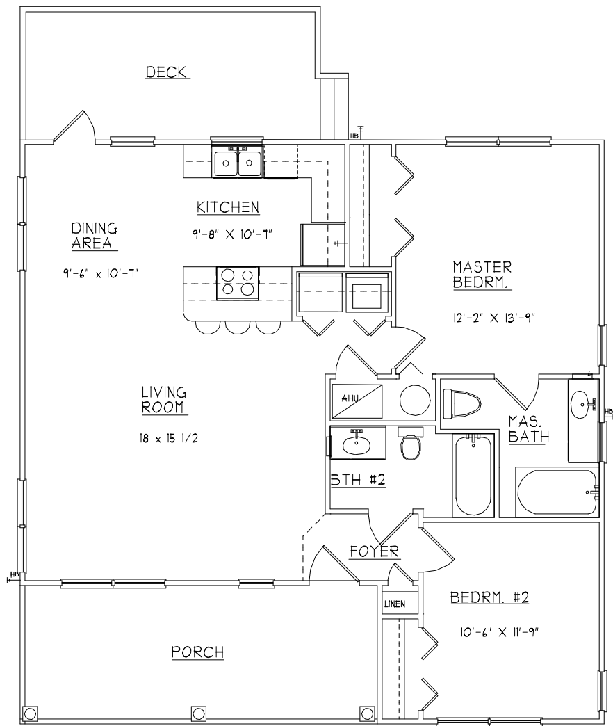
FLOOR PLAN
