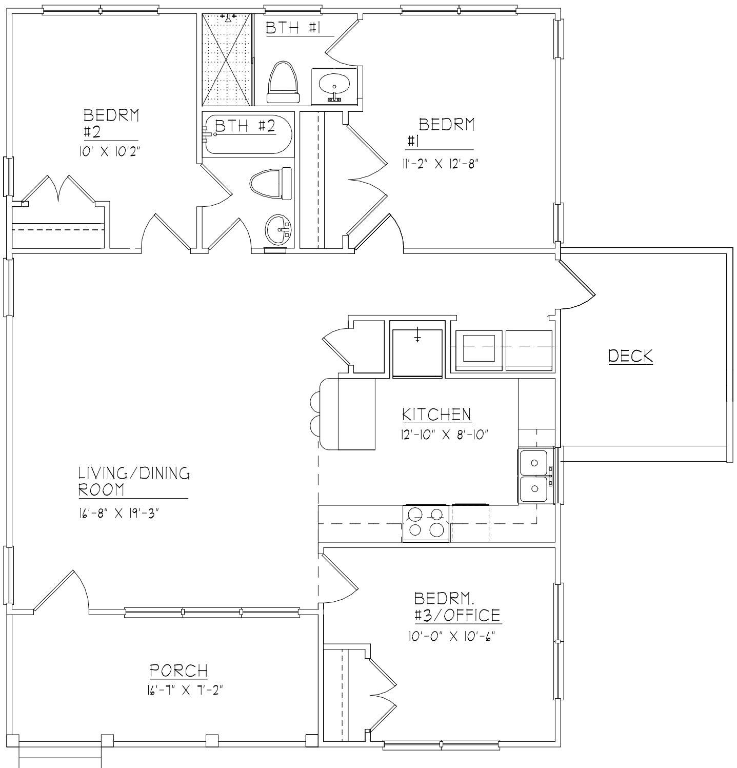
FLOOR PLAN 1079 SQ. FT.
