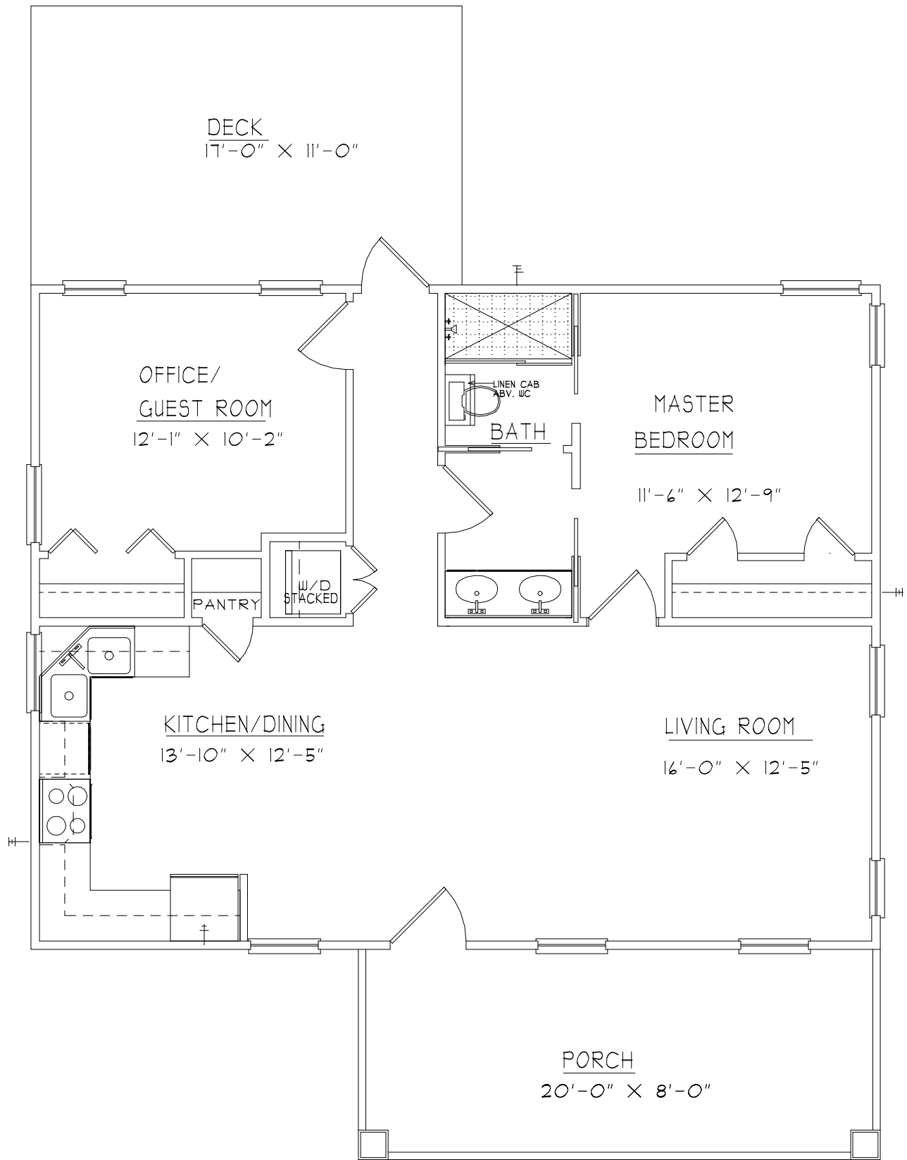
FLOOR PLAN 884 SQ. FT.
